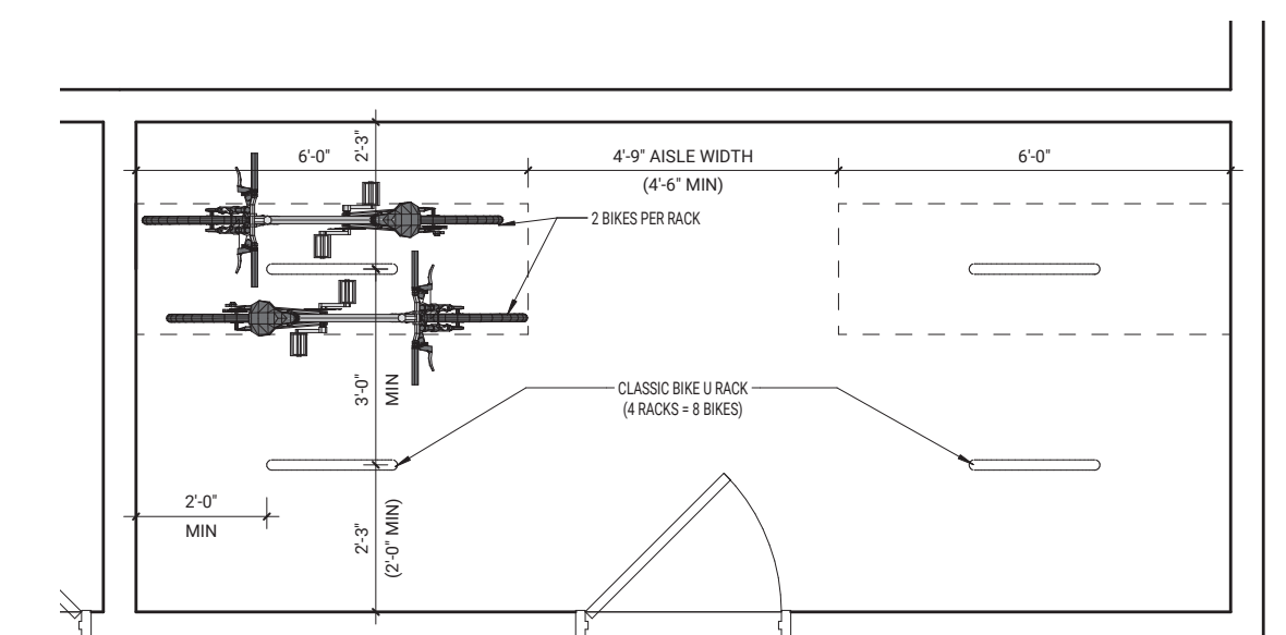
BIKE ROOM LAYOUT
