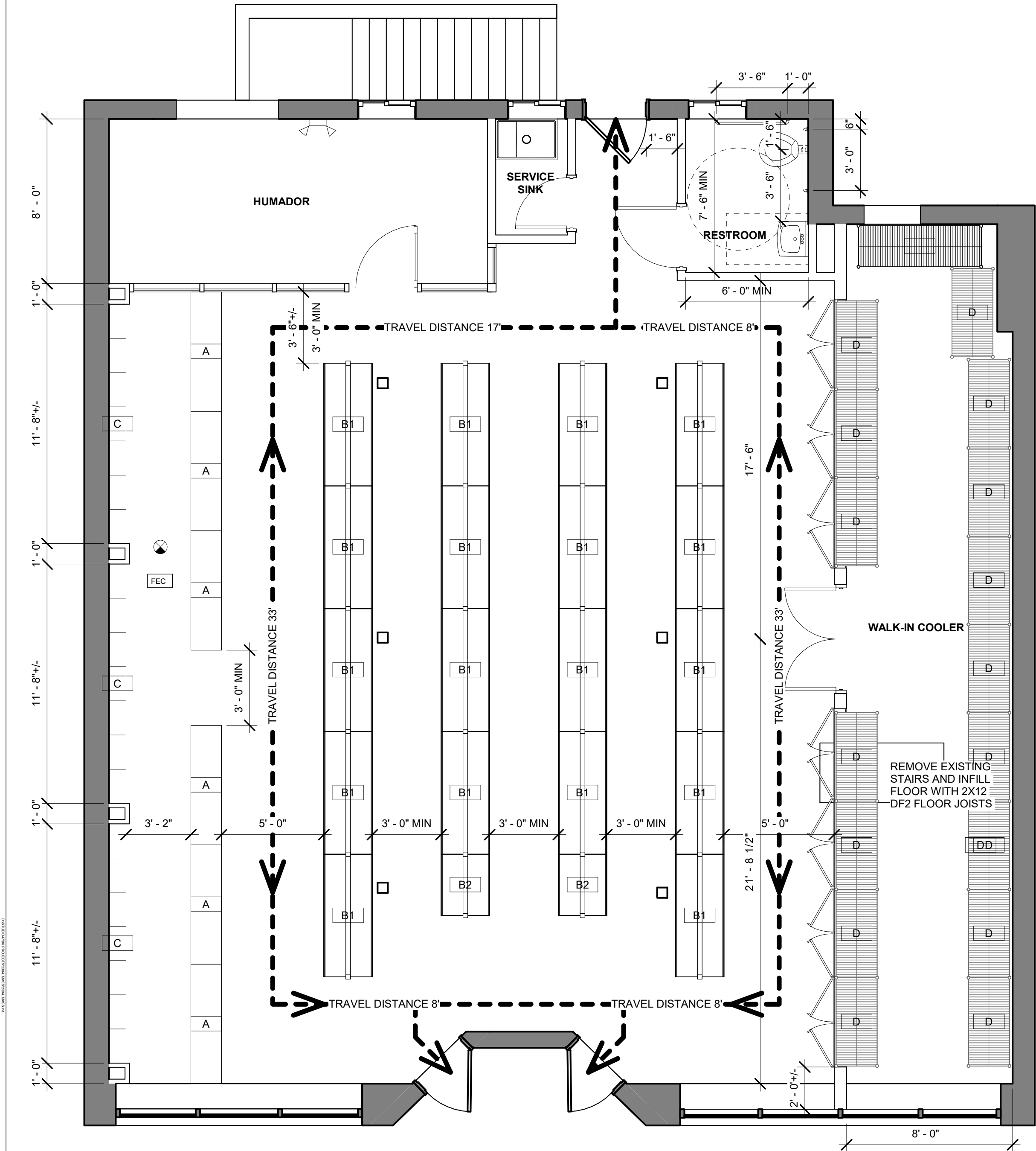
1 FLOOR PLAN 1/4" = 1'-0"
