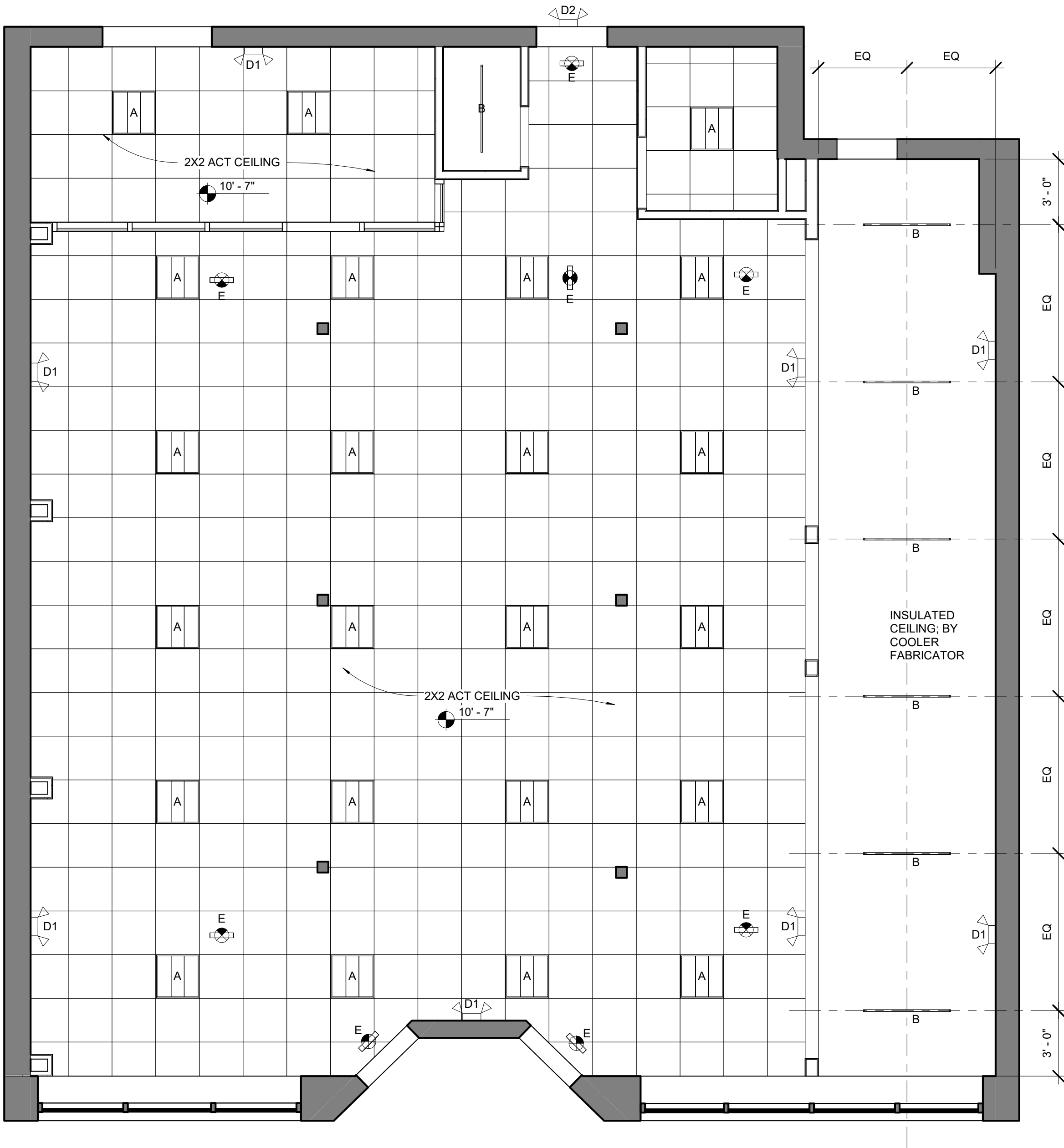
2 REFLECTED CEILING PLAN 1/4" = 1'-0"
