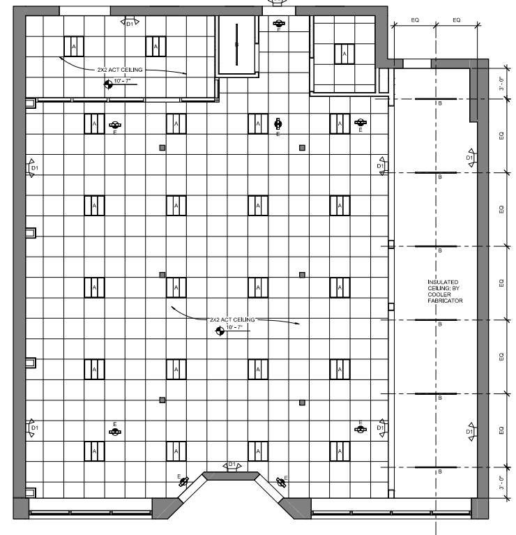
2 REFLECTED CEILING PLAN 1/4" = 1'-0"
