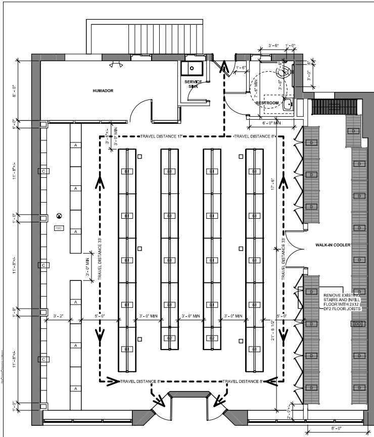
1 FLOOR PLAN 1/4" = 1'-0"
