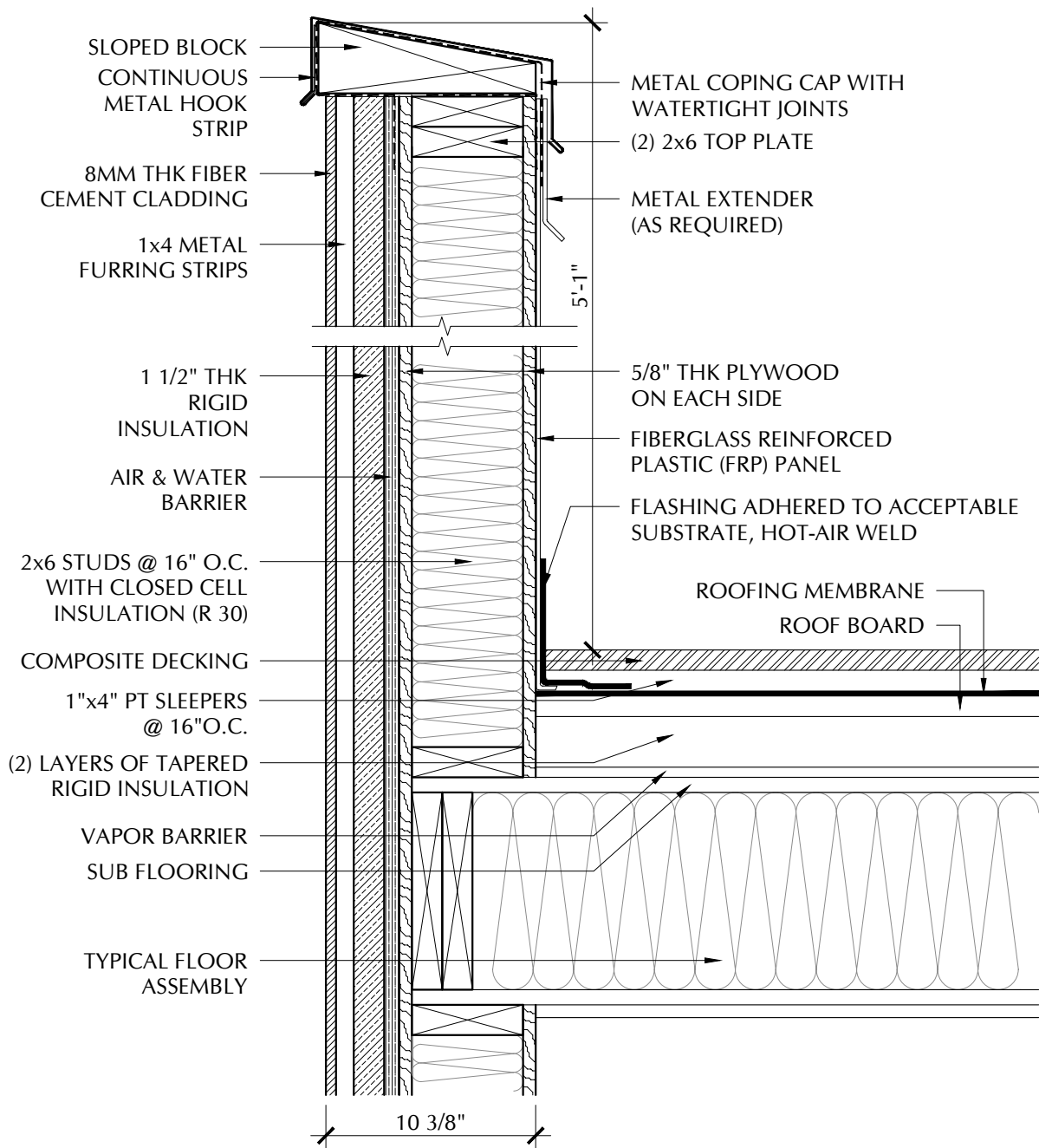
1 PROPOSED PARAPET WALL DETAIL - TYPICAL
